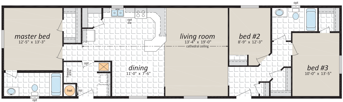
CJ-3005 , 20' x 76' - 1,520 sq. ft.
