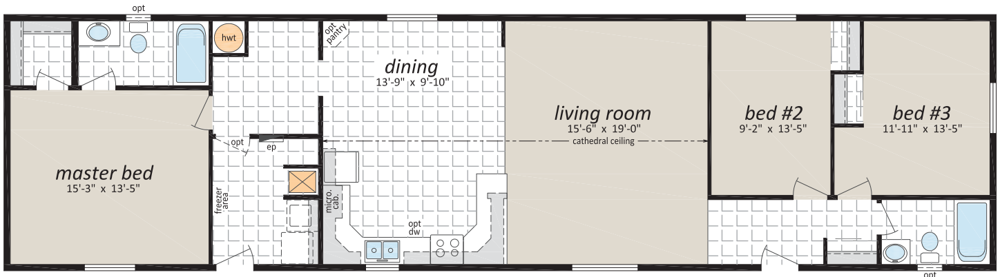
CJ-3000 , 20' x 76' - 1,520 sq. ft.
