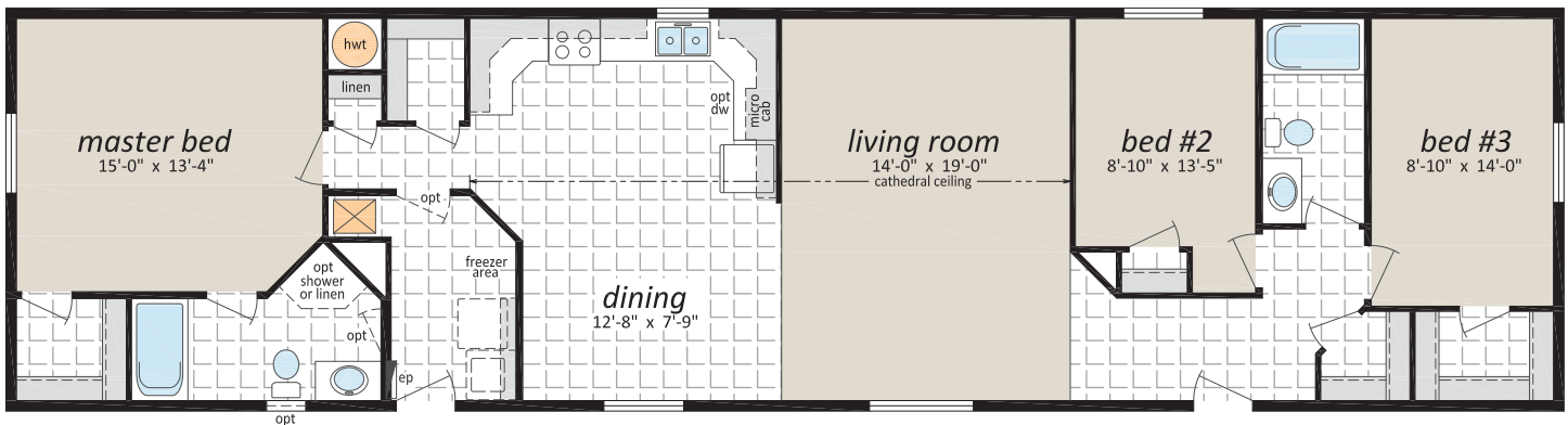
Optional Kitchen Layout
